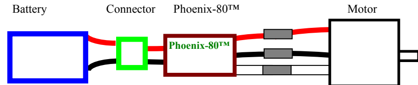
Fig 1: Motor wiring diagram
